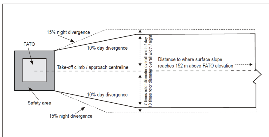
Figure 4-2. Take-off climb/approach surface width
