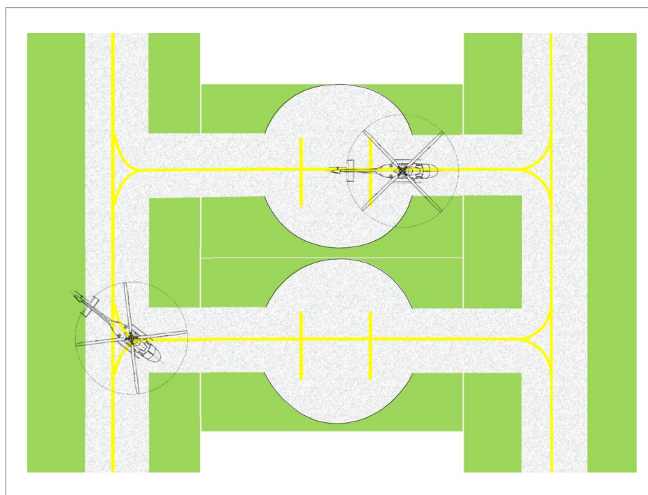
Figure 3-6. Ground taxi-through stands (with taxiway/ground taxi-route) simultaneous use
