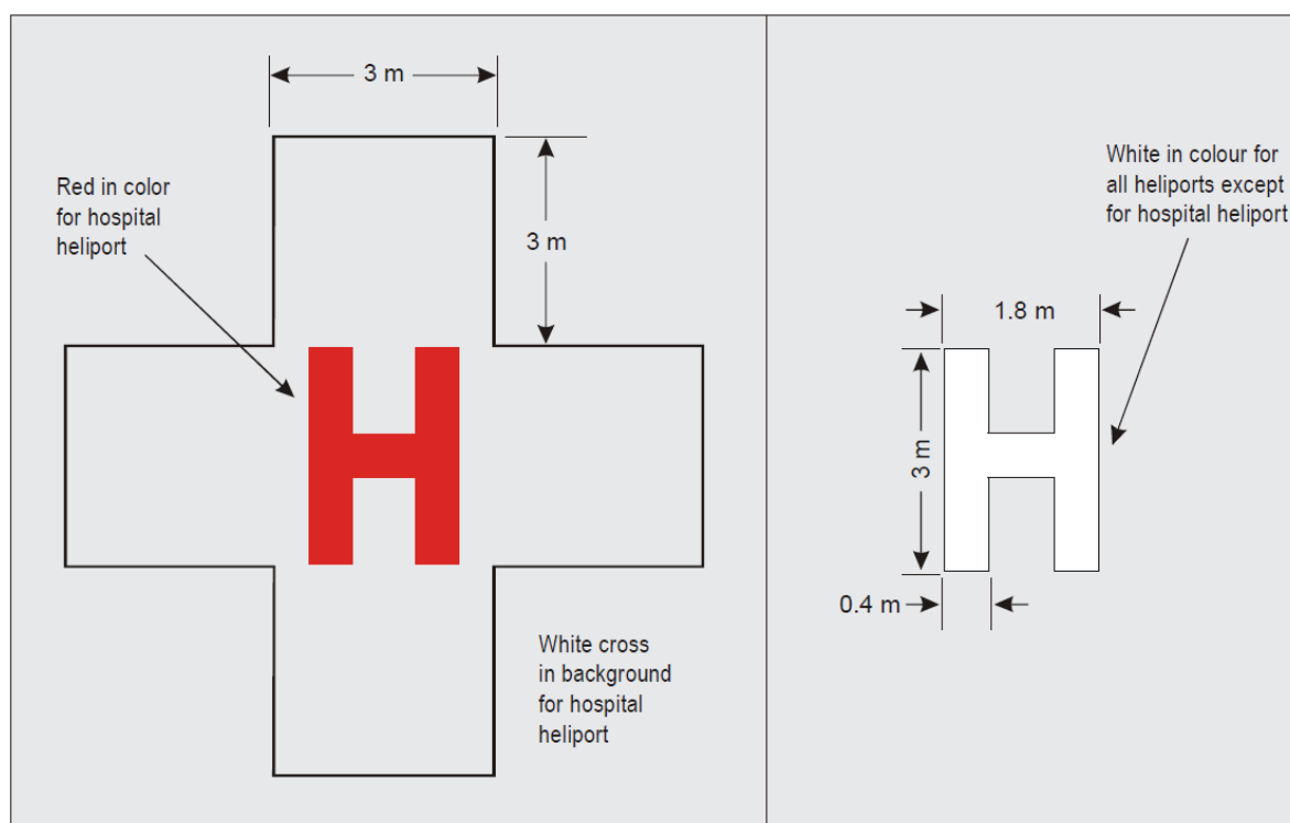
Figure 5-4. Hospital heliport identification and heliport identification marking
