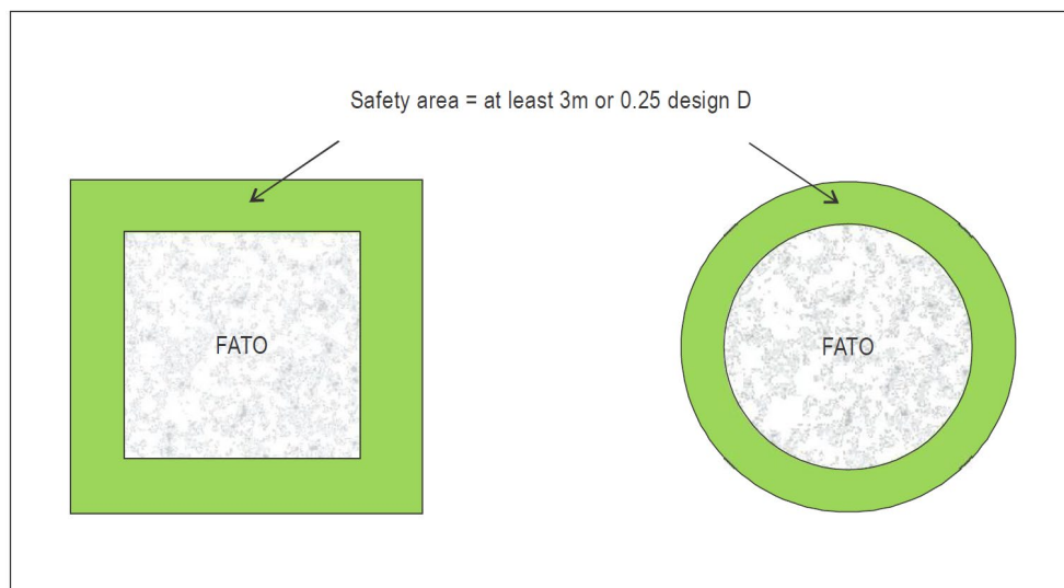
Figure 3-1. FATO and associated safety area
