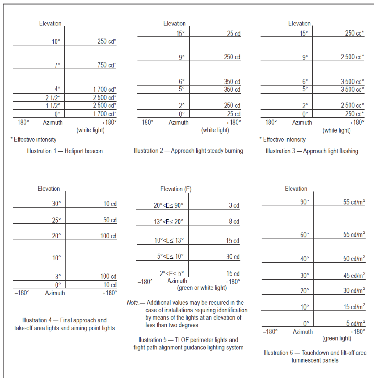
Figure 5-12. Isocandela diagrams
