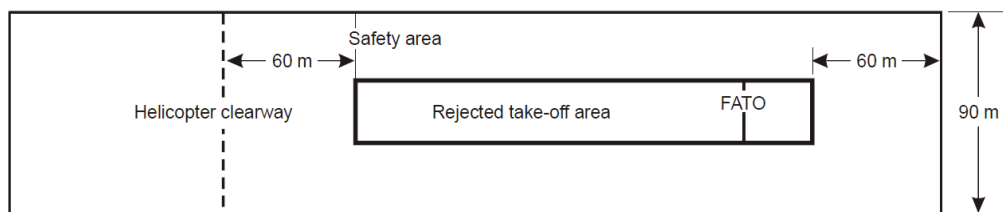
Figure A-1. Safety area for instrument FATO
