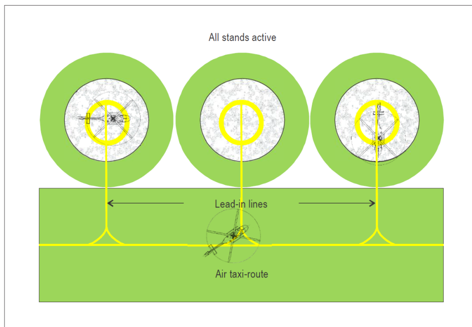
Figure 3-5. Turning stands (with air taxi-routes) — simultaneous use
