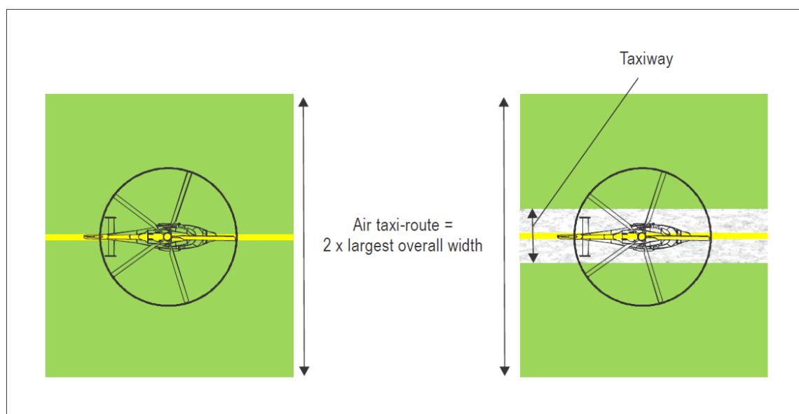
Figure 3-4. Helicopter air taxi-route and combined air taxi-route/taxiway
