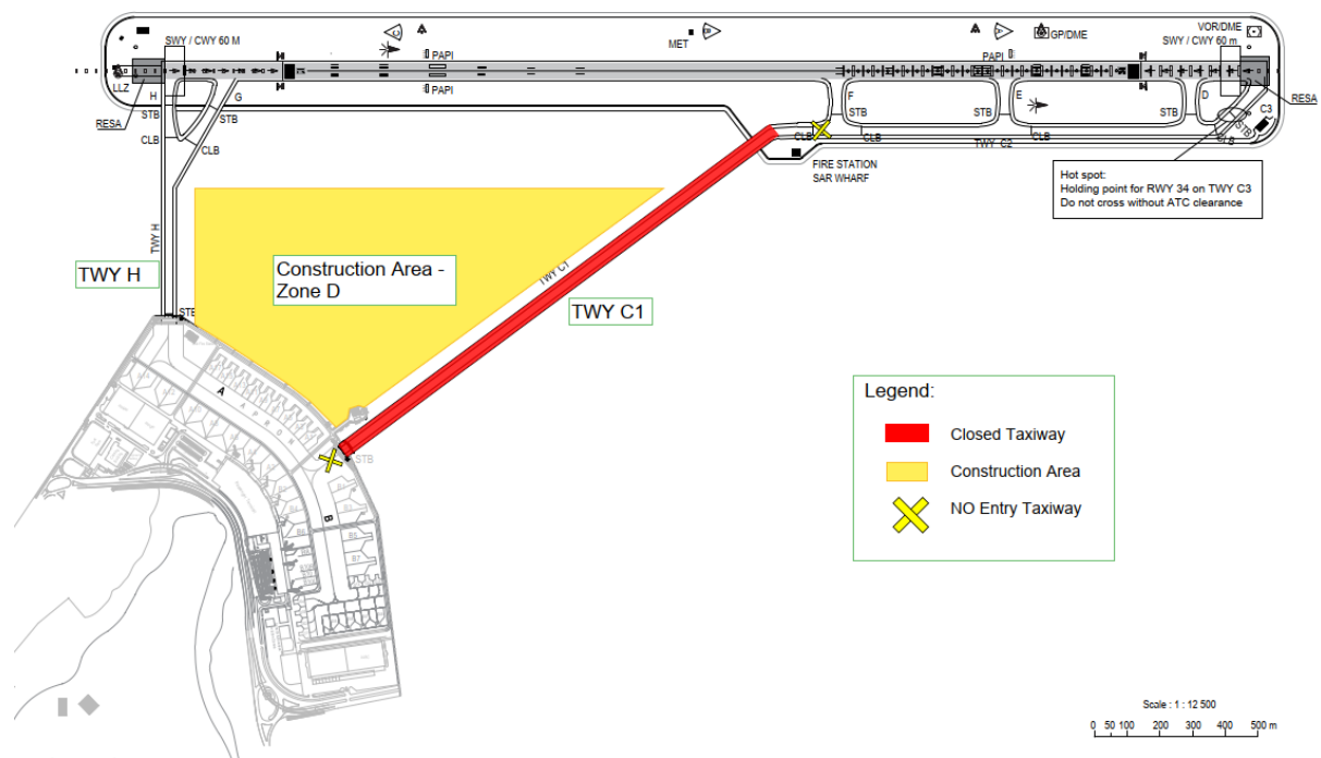
Figure 1. Closure of Taxiway C1
