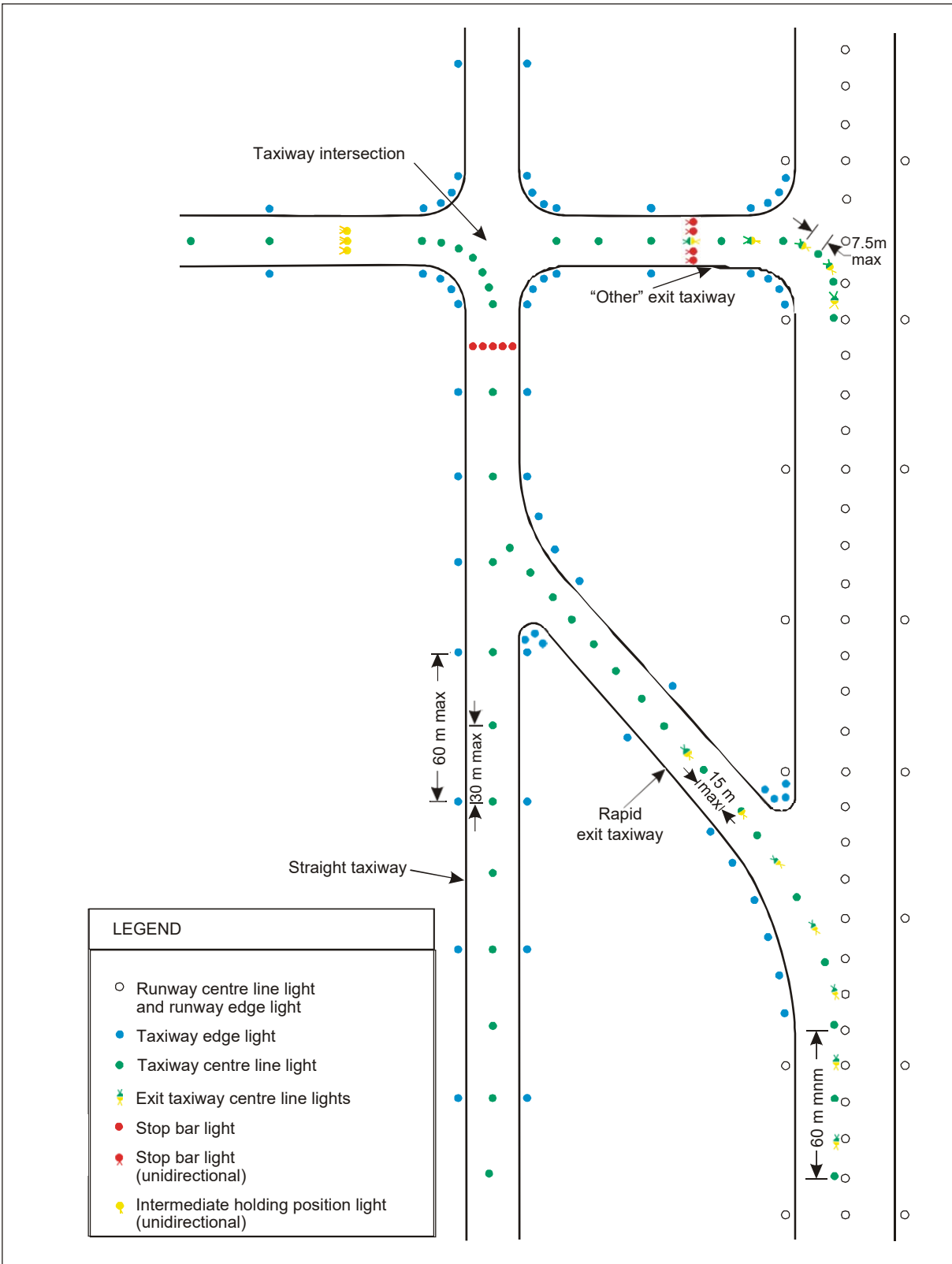
Figure 5-26. Taxiway lighting
