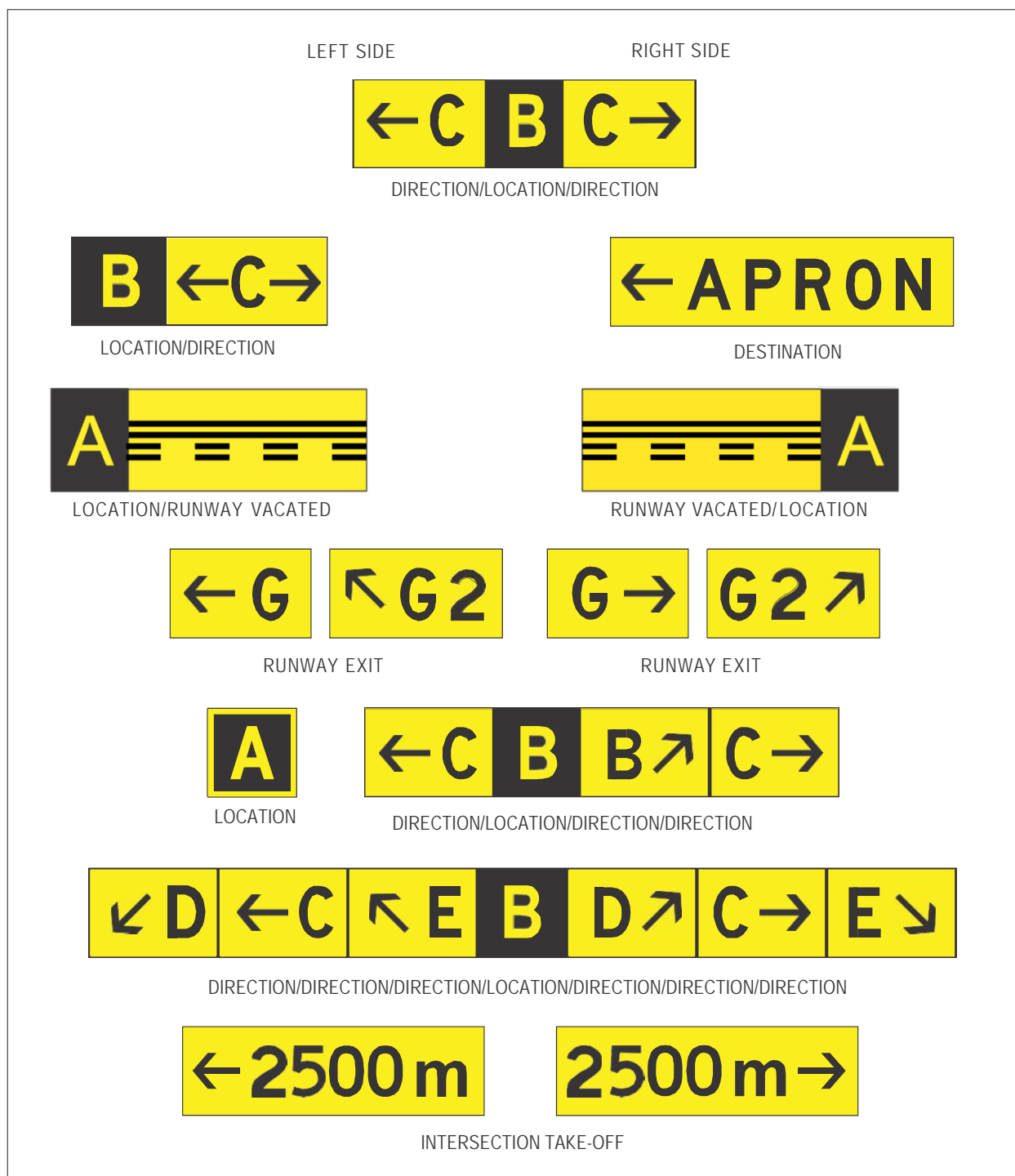
Figure 5-31. Information signs
