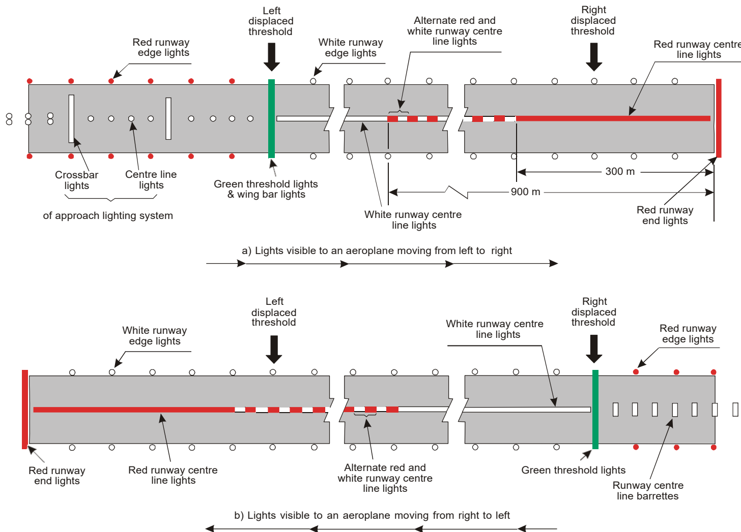
Figure 5-23. Example of approach and runway lighting for runway with displaced thresholds
